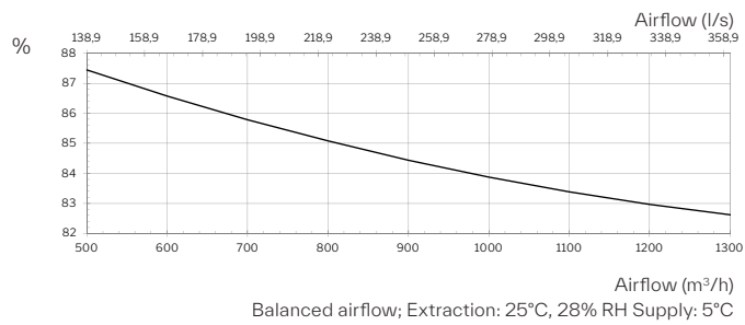
Temperature efficiency, acc. to EN 308
