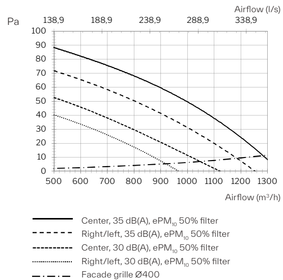
External pressure loss - Extract Air
